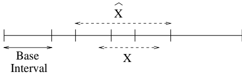
Figure 4: Illustration for Lemma 2
